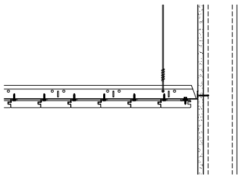
FLOATING OPEN REVEAL
